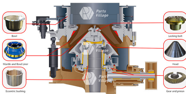
HP SERIES MULTI-CYLINDER CONE CRUSHER
