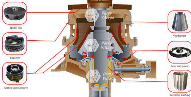
SINGLE-CYLINDER CONE CRUSHER
